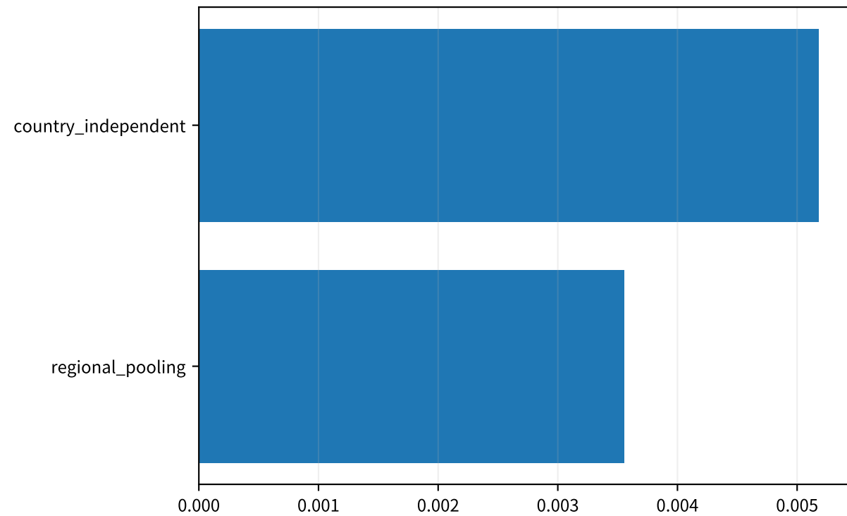
CommonQuintileMonotonicity
