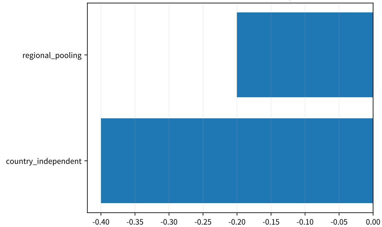
CommonQuintileMonotonicity
