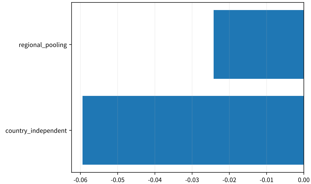
CommonQ5MinusQ1MaxDrawdown
