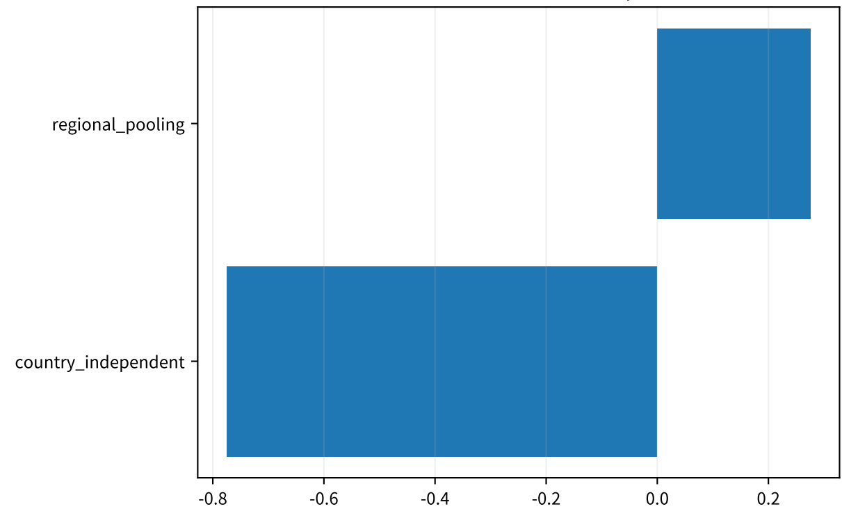
CommonQ5MinusQ1MaxDrawdown
